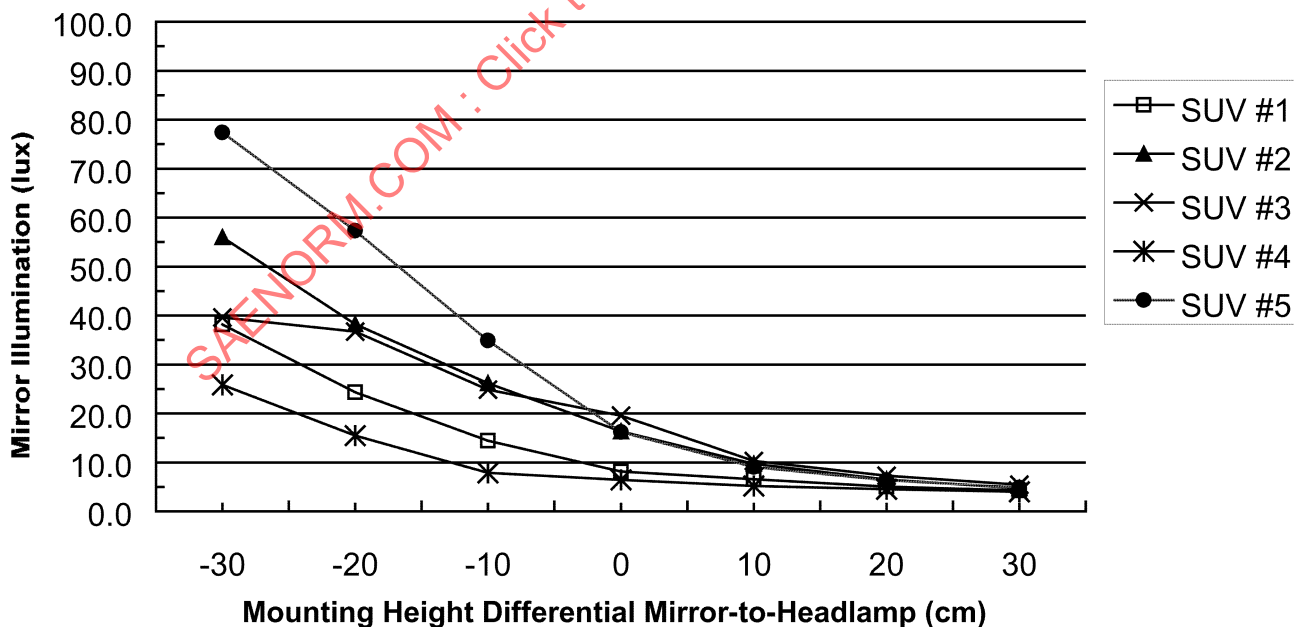
FIGURE 3—9007 SIDE MIRROR ILLUMINANCE AT 15 m FOLLOWING DISTANCE— SUV VEHICLES
