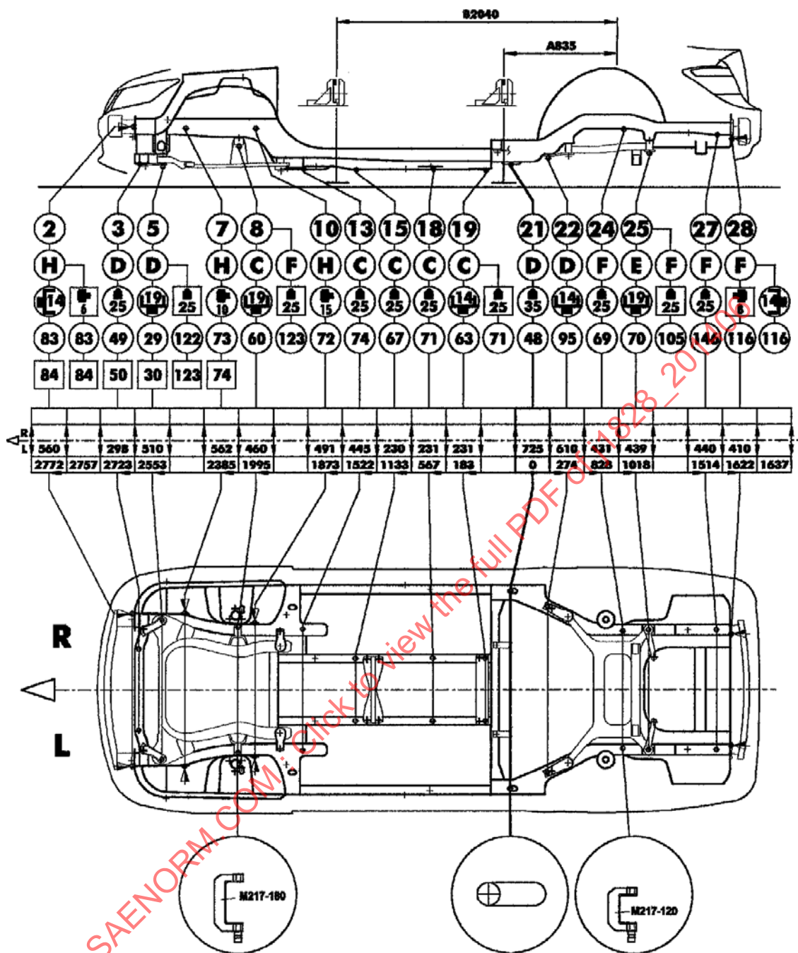
FIGURE 8 - SYMBOLS DEFINING DIRECTION OF VIEW MEASURING POINT SYMBOLS; IN-PLANE DIMENSIONS
