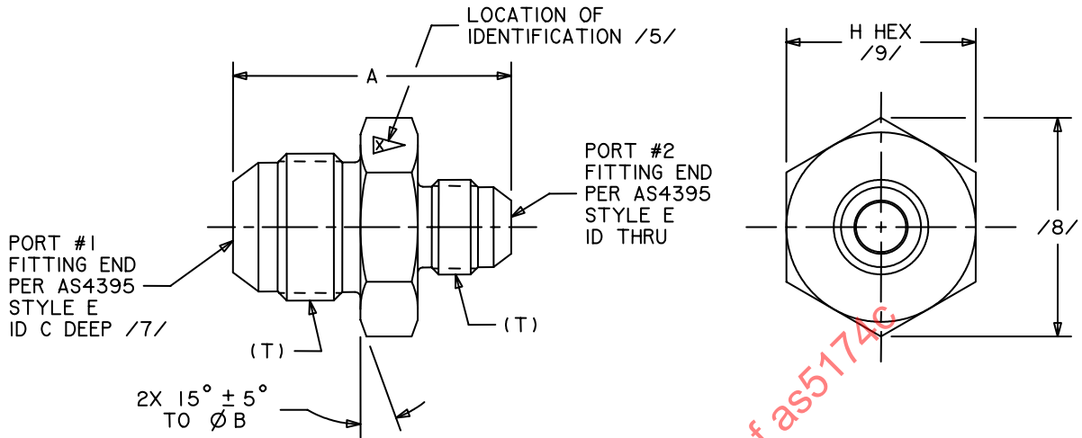
FIGURE 1 – FITTING, UNION AND REDUCER
