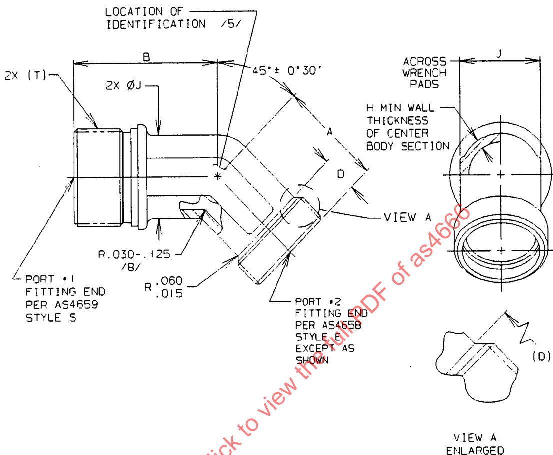
FIGURE 1 - ELBOW, 45°
