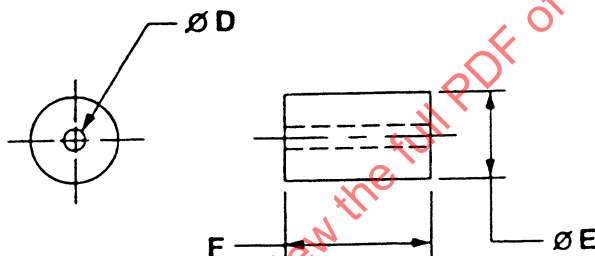
FIGURE 2 - FERRULE
