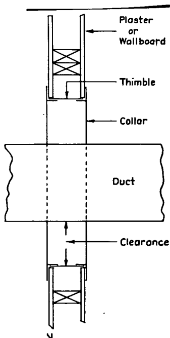
Figure 4. An arrangement for passing ducts through combustible walls or partitions as specified in par. 143 e.
