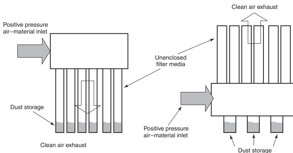
FIGURE A.9.3.3.2.6.4 Two Typical Enclosureless Dust Collectors.
