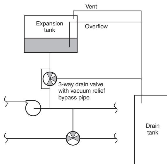
FIGURE A.10.6.3(b) Expansion Tank Isolation Using a Three-Way Valve.
