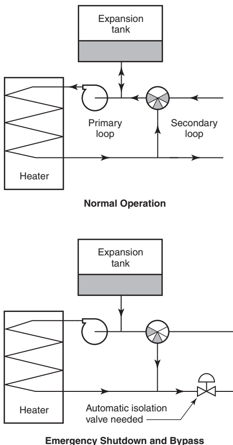
FIGURE A.10.1.1(5)(b) Three-Way Valve on Return Leg.
