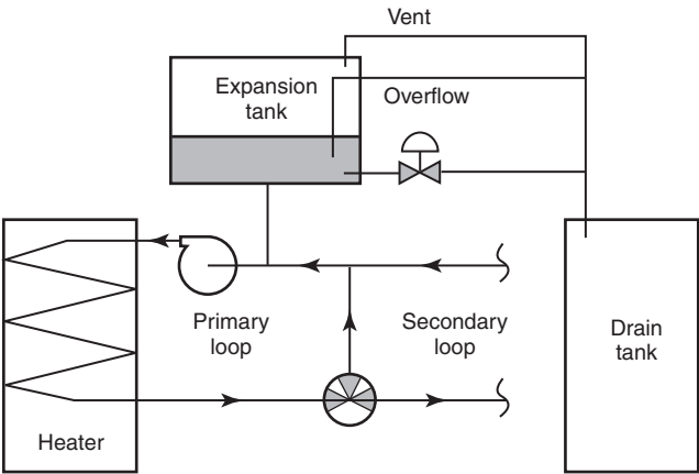
FIGURE A.10.1 Typical Thermal Oil Heating System Components.
