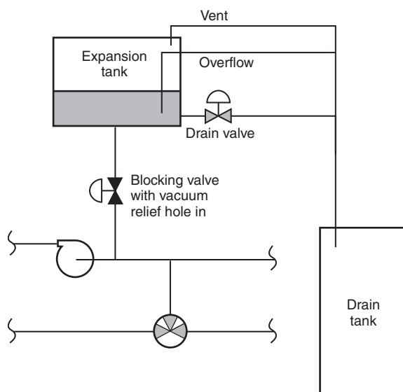
FIGURE A.10.6.3(a) Expansion Tank Isolation Using Drain and Blocking Valves.
