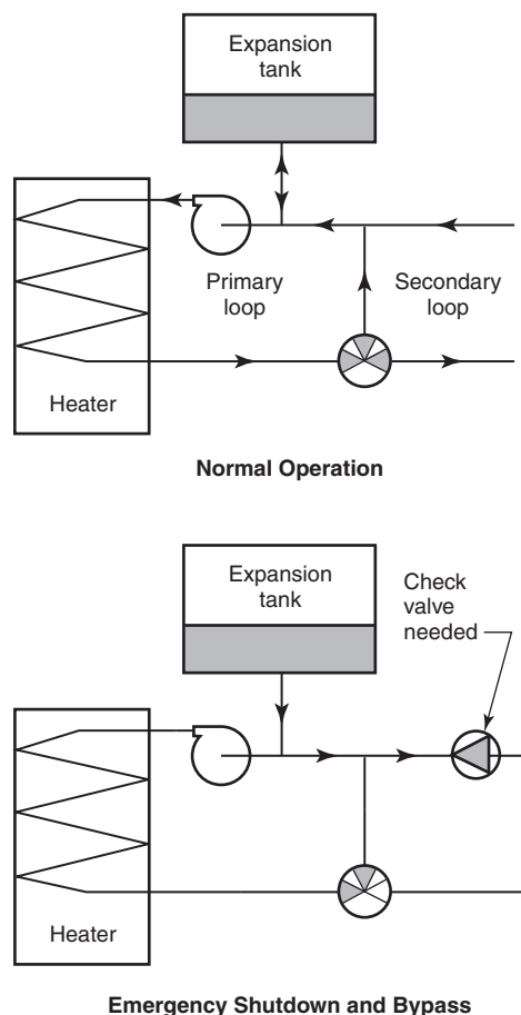
FIGURE A.10.1.1(5)(a) Three-Way Valve on Supply Leg.
