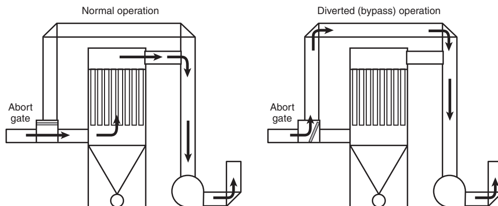
▲ FIGURE A.9.8.5(2)(b) Diversion of Sparks with a Single Abort Gate Up-Stream of Dust Collector.
