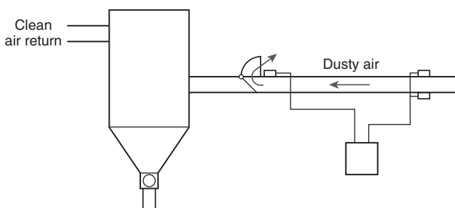
FIGURE A.9.3.5.4(a) Spark Detection and Abort Gate on Inlet Duct to the Dust Collector.
