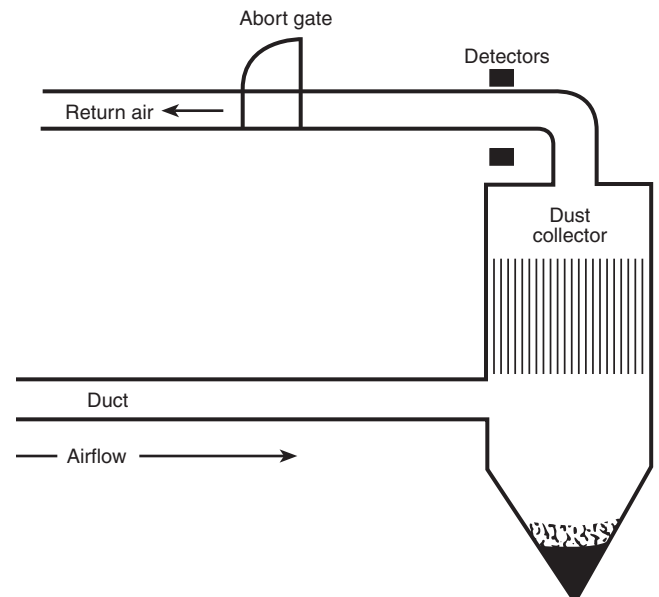
Δ FIGURE C.1.1.1 Spark Detectors and Abort Gate.
