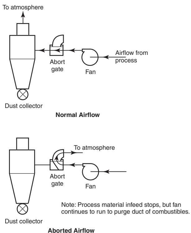
FIGURE A.9.8.5(2)(a) Aborting of Positive Pressure Systems.
