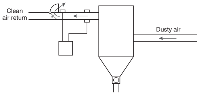
FIGURE A.9.3.5.4(b) Spark Detection and Abort Gate on Clean Air Side of the Dust Collector.
