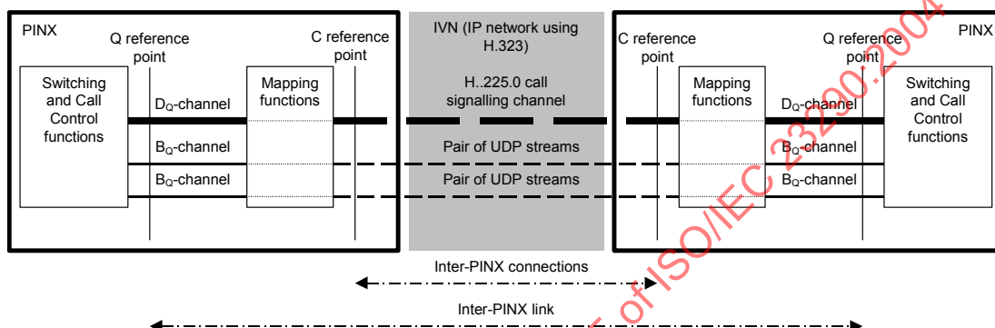
Figure 2 — H.323 as intervening network (IVN)
