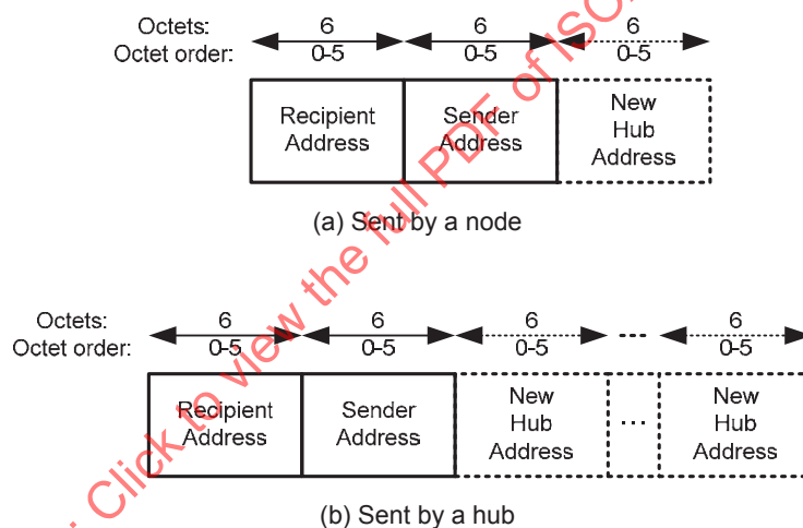
Figure 33—Frame Payload format for Disconnection frames
