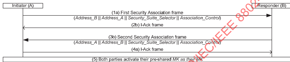
Figure 102 —MK pre-shared association procedure
