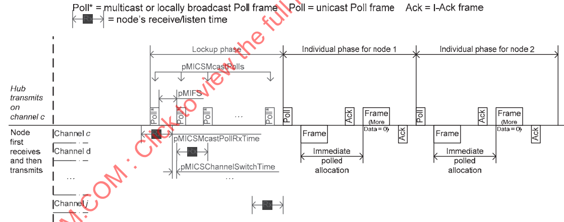
Figure 84—Multicast poll aided connected discovery and frame exchange in MICS band
