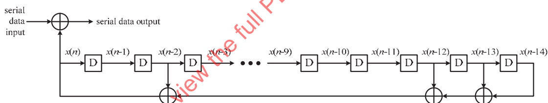
Figure 132 —Block diagram of an additive or synchronous scrambler
