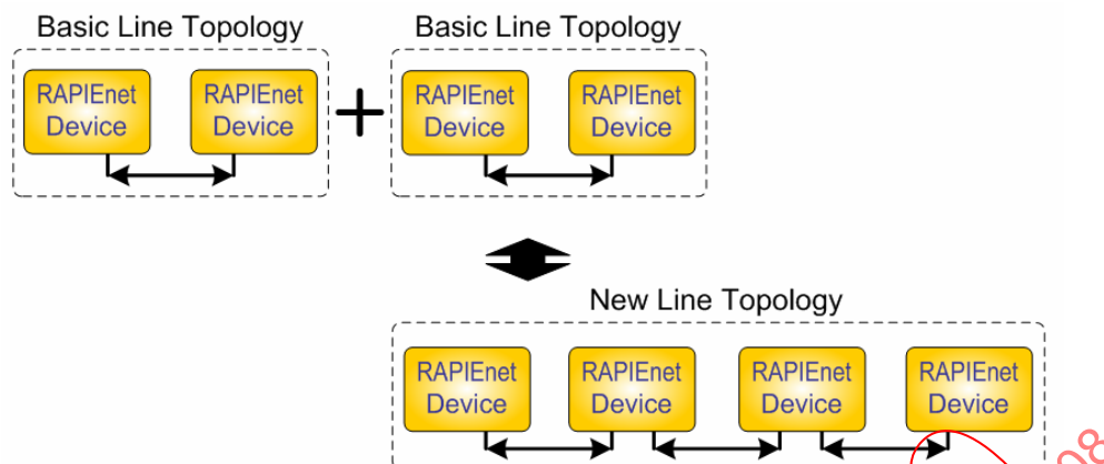
Figure 5 – Line topology
