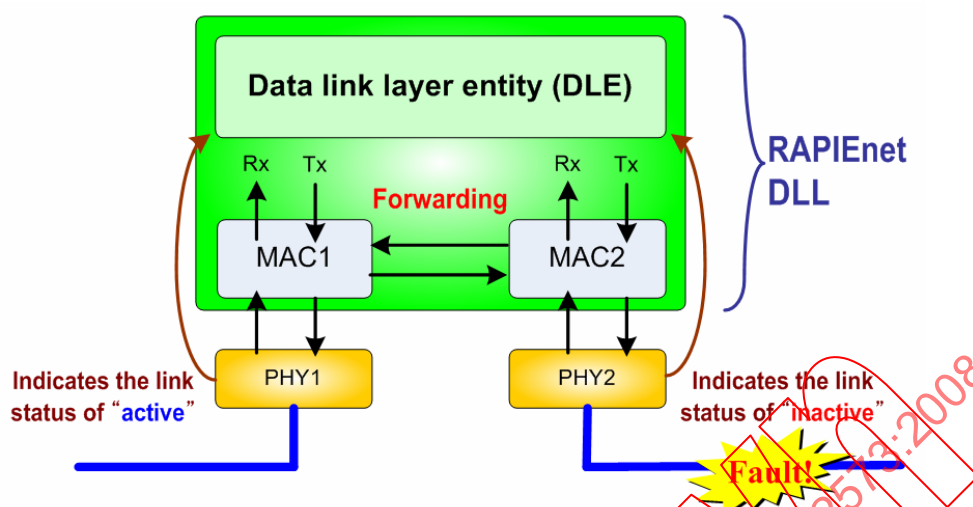
Figure 4 – Link status information
