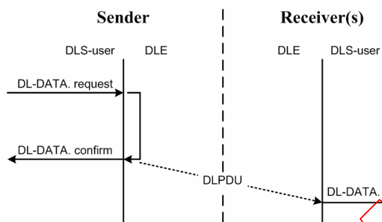
Figure 13 – Sequence diagram of DL-DATA service
