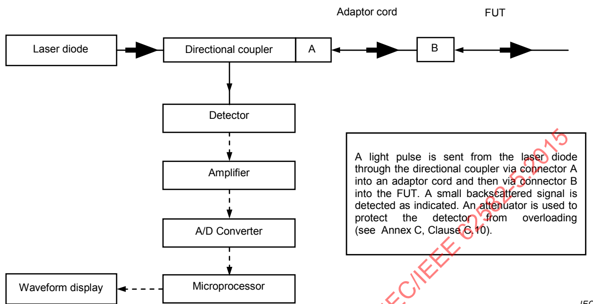
Figure 1 – Block functions of the OTDR
