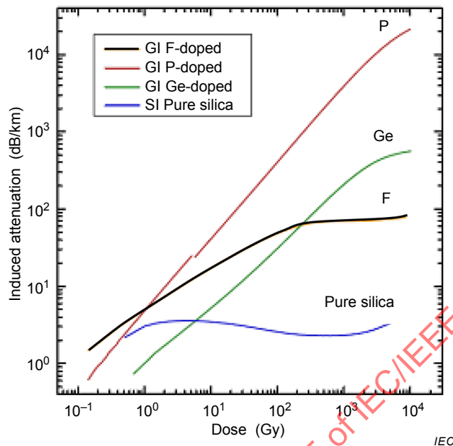
Figure B.2 – RIA of different fibre types 2
