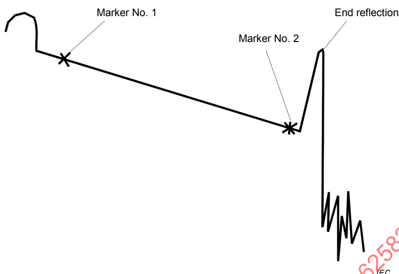
Figure C.1 – Markers for measuring attenuation
