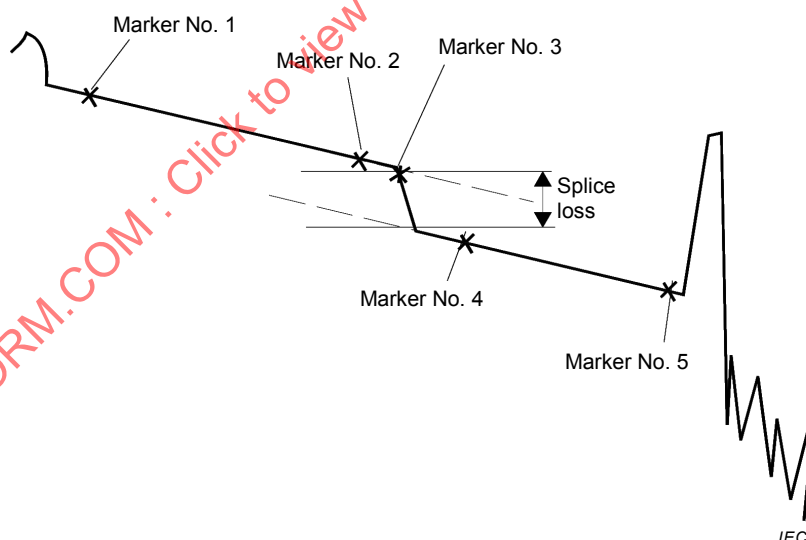
Figure C.2 – Markers for measuring splice loss
