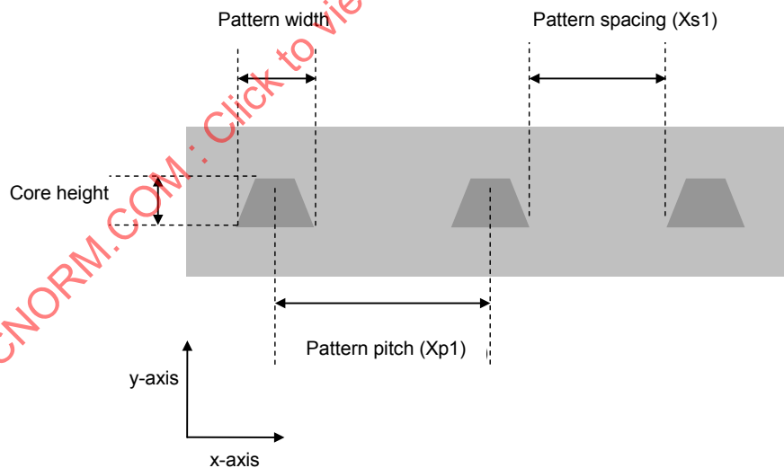
Figure A.1 – Pattern pitch and objects of measurement (an example of single layer)
