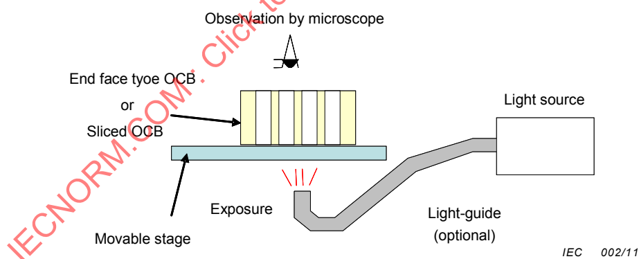
Figure 2 – Example of sample set-up for observation of core shape (end face I/O type OCB or a sliced sample)
