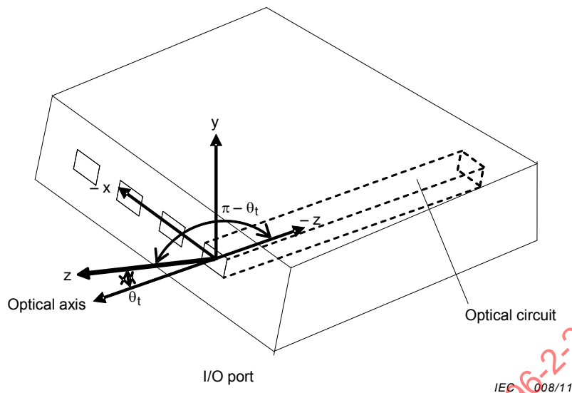
Figure 7 – Misalignment angle of I/O ports in end face I/O type OCB
