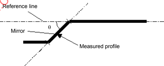
Figure 12 – Example of the profile at a mirror portion using a confocal microscope
