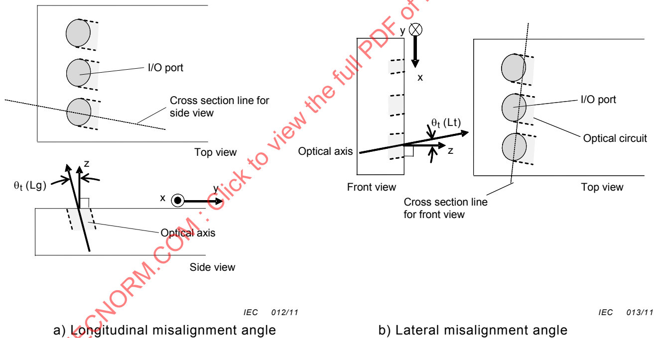
Figure 10 – Parameters for misalignment angle in surface I/O type OCB
