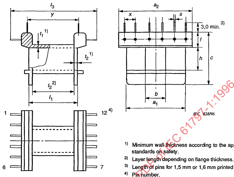
Figure 9 – YEx 2 coil formers for printed wiring board mounting, level mounting style
